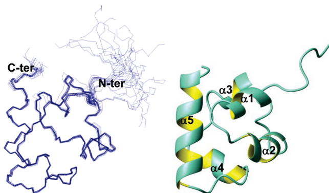
FIGURE 2: (Left panel) Overlay on the backbone atoms (residues 29–85) of 20 Ship2-Sam NMR conformers. The final structure calculation includes 989 nonredundant distance constraints (263 intrasidue, 240 short-range, 242 medium-range, and 244 long-range) and 282 angle constraints. (Right panel) Ribbon drawing of one Ship2-Sam NMR conformer (number one). It contains the following secondary structure elements: \alpha 1 (residues 30–34), \alpha 2 (residues 39–46), \alpha 3 (residues 53–56), \alpha 4 (residues 61–66), and \alpha 5 (residues 72–84).
