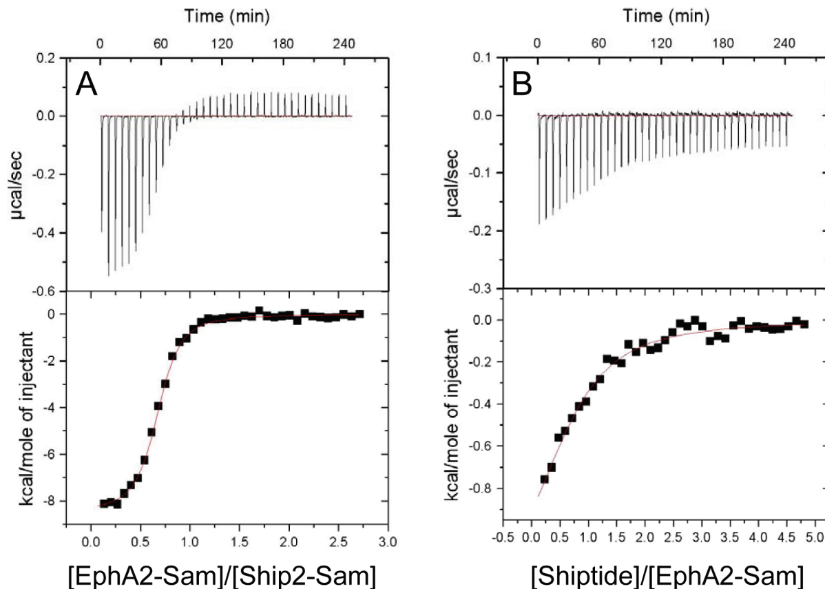
FIGURE 5: ITC studies. (A) The raw and integrated data are shown in the upper and lower panels, respectively. In the lower panel, solid squares represent data from the EphA2-Sam (300 \mu M) titration into Ship2-Sam solution (25 \mu M); the solid red line represents the fit to a single binding site model. (B) Calorimetric curve representing the EphA2-Sam (50 \mu M) titration with the Shiptide peptide (1 mM).
