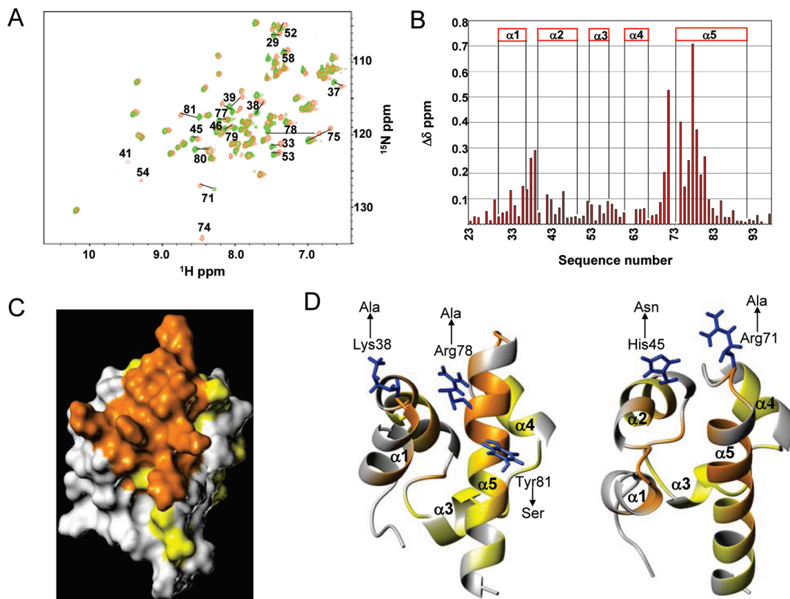
FIGURE 4: (A) Superposition of [ 1 H, 15 N]-HSQC spectra of EphA2-Sam (200 \mu M concentration) in its unbound form (green) and after complex formation with Ship2-Sam (400 \mu M) (brown). (B) Plot of normalized chemical shift deviations ( \Delta\delta = [(\Delta H_N)^2 + (0.17 \times \Delta^{15}N)^2]^{1/2} ) versus residue number. The highest normalized chemical shift deviations ( \Delta\delta values >0.1 ppm) are observed for residues W33, I37, K38, M39, Y42, F46, R71, L72, H75, Q76, K77, R78, I79, A80, and Y81. Minor changes ( 0.05 < \Delta\delta values <0.1 ppm) affect amino acids T29, L34, T43, H45, T52, A53, E55, V57, V58, Q59, T61, D64, I65, K66, S82, L83, G85, and D88. Data are not shown for residues N62 and D63 (unassigned); G74, Q41 (their peaks only appear in the spectrum of the complex). (C) Surface representation of EphA2-Sam (conformer number 1, pdb i.d.: 2E8N, from RIKEN Structural Genomics Initiative) (in the same orientation as in D, left panel); residues exhibiting the greatest normalized chemical shift deviations ( \Delta\delta values >0.1 ppm) are colored in orange, and those presenting minor changes ( 0.05 < \Delta\delta values <0.1 ppm) are reported in yellow. (D) EphA2-Sam mutants. Ribbon representation of EphA2-Sam (colored as in panel C). The side chains of the mutated residues are also shown together with the corresponding mutations.
