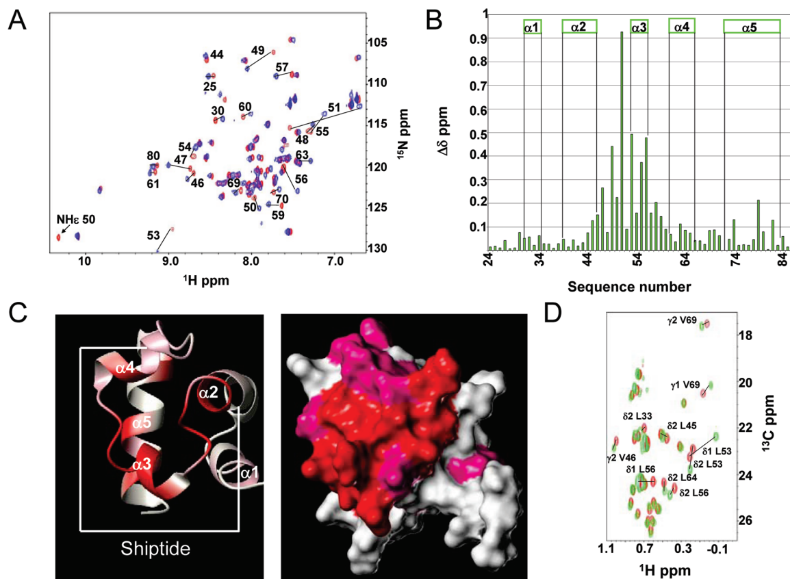
FIGURE 3: (A) Comparison of [^1\text{H}, ^{15}\text{N}] -HSQC spectra of Ship2-Sam (100 \mu\text{M} ) in its apo form (red) and after the addition of EphA2-Sam (400 \mu\text{M} ) (blue). (B) Histogram showing normalized chemical shift deviations ( \Delta\delta = [(\Delta H_N)^2 + (0.17 \times \Delta^{15}\text{N})^2]^{1/2} ) as a function of the residue number. Residues L45, V46, H47, G49, W50, D51, L53, E54, F55, L56, S57, D58, I59, D63, H74, L79, and L82 present normalized deviations with values higher than 0.1 ppm. \Delta\delta values in between 0.05 and 0.1 ppm are observed for the following residues: S30, A31, W32, R34, G44, N48, D52, T60, E61, L64, E65, E66, A67, V69, Q70, D71, and D80. (C) Residues with normalized chemical shifts ( \Delta\delta values) greater than 0.1 ppm and included in between 0.05 and 0.1 are colored in red and pink, respectively, on the 3D solution structure of Ship2-Sam (conformer number 1) in its ribbon (left panel) and surface (right panel) representations. The peptide region used for our studies is highlighted in the left panel. (D) [^1\text{H}, ^{13}\text{C}] -HSQC spectra of selective Leu- ^{13}\text{CH}_3^{\delta 1,2} /Val- ^{13}\text{CH}_3^{\gamma 1,2} labeled Ship2-Sam (50 \mu\text{M} ) in the absence (red) and presence (green) of EphA2-Sam (150 \mu\text{M} ).
