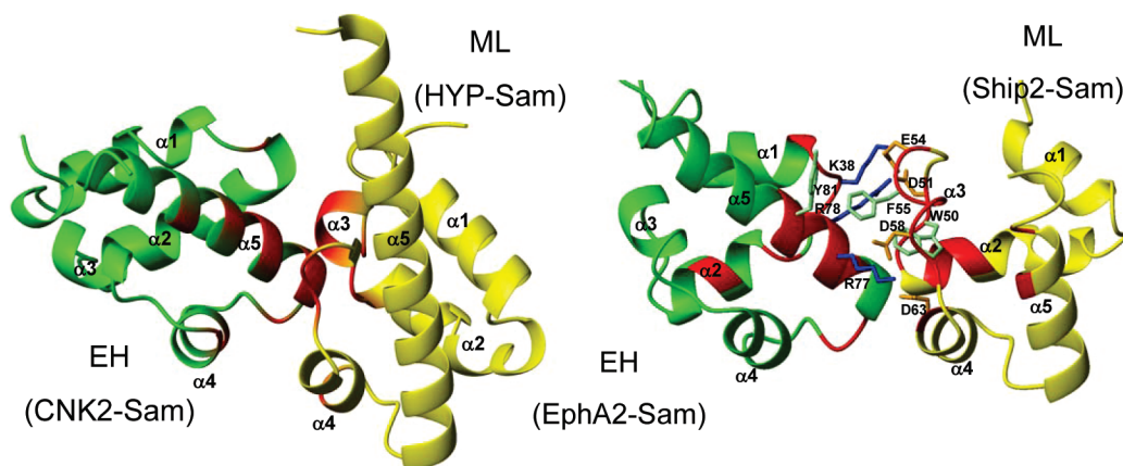
FIGURE 6: (Left panel) Crystal structure of the complex between CNK2-Sam (green) and HYP-Sam (yellow) (pdb code: 3BS5 (11)). Residues contributing to the ML and EH interfaces (11) have been colored in red on the ribbon representations of the two molecules. (Right panel) Model generated with Haddock 1.3 (25) of the Ship2-Sam/EphA2-Sam complex (solution with the lowest Haddock score). Residues with the largest chemical shift perturbations, according to our NMR binding studies, have been reported in red. The side chains of amino acids, which are involved in interactions at the dimer interface are also shown.
